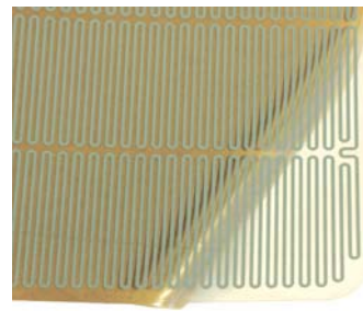
Detail of the part heating (Fixation by adhesive face)
